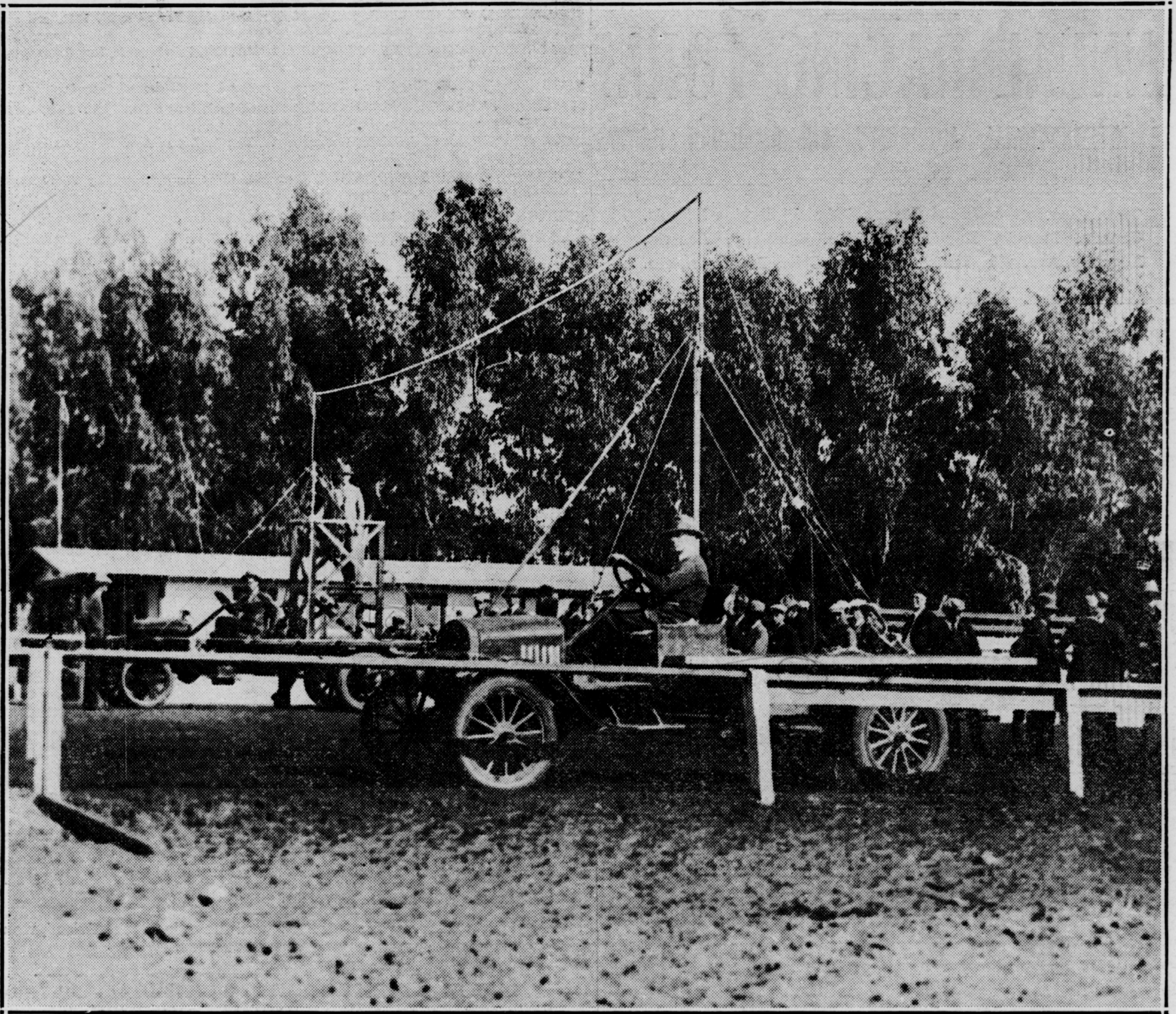
The gate and trucks on which it is mounted in position. The starter's platform is mounted on the outside truck. Starter controls the speed, stopping and starting of trucks, chauffeurs only guiding them. Gate itself is same as gates now in use. Outside truck may be speeded up rounding turns. Horses line up just after post parade and walk behind the webbing to the starting point and are started without pausing for a standing break. Starter uses his own judgment as to how close to actual starting point horses shall be started, but within forty to twenty-five feet of the post.
